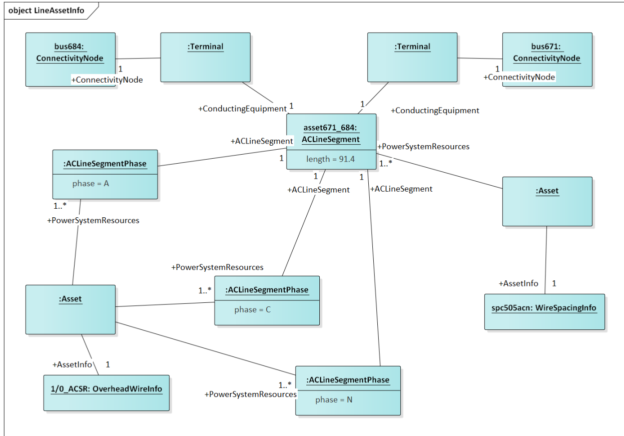
Figure 26: The two-phase ALineSegment impedance defined by sharing wire and spacing data from a catalog. Each ALineSegmentPhase links to an OverheadWireInfo instance via the Asset instance. If the neutral (N) is present, we have to specify its wire information for a correct impedance calculation. In this case, ACN all use the same wire type, but they can be different, especially for the neutral. Similarly, the WireSpacingInfo associates to the ALineSegment itself via a separate Asset instance. These Asset instances only exist when the catalog data is used, so cardinalities are 1 for AssetInfo and 1..* for PowerSystemResources.
